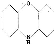
Phenoxazin.
